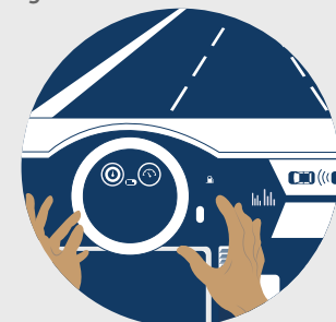
Supervised Learning
