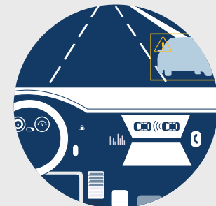
Computer Vision
